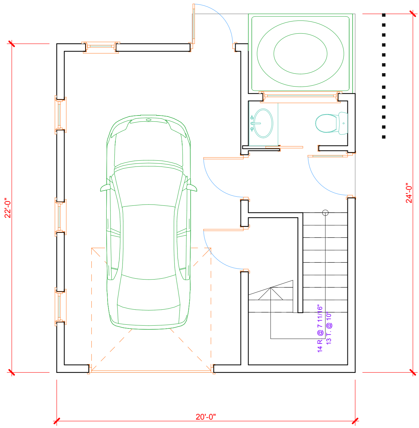
01 First Floor Plan SCALE: 1/4" = 1'-0"
